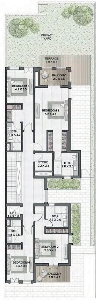
1. FLOOR
