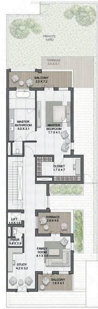
2. FLOOR
